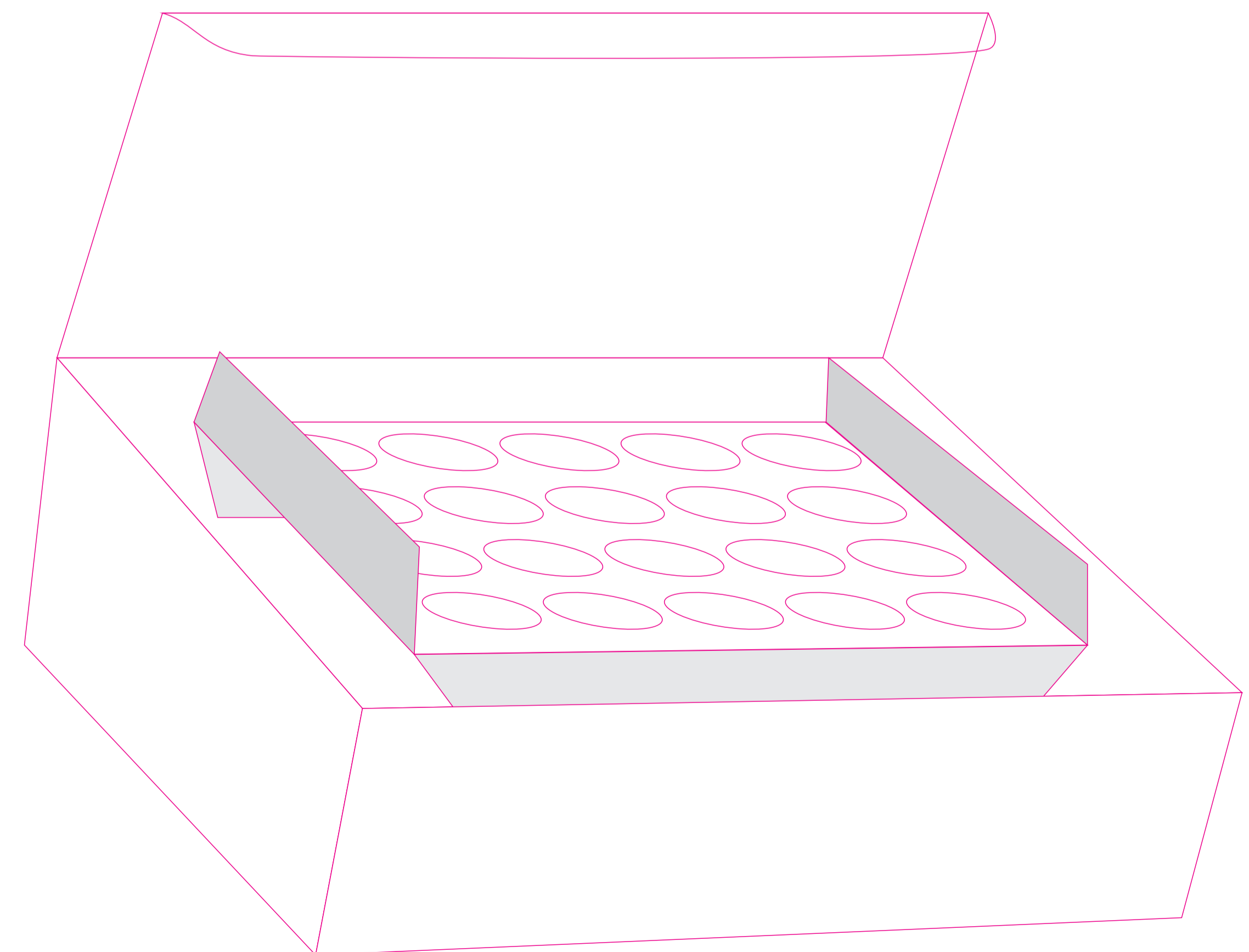
Position of partition in a carton
