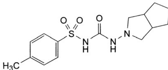
STRUCTURAL FORMULA GLICLAZIDE
